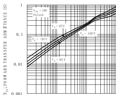
Fig. 10 Forward Transfer Admittance
