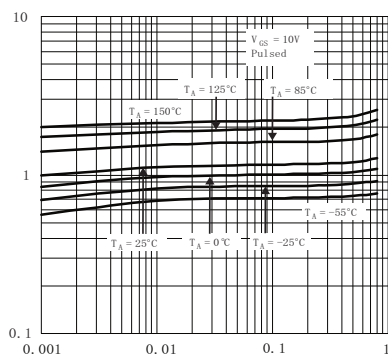
Fig. 4 Static Drain-Source On-Resistance vs. Drain Current
